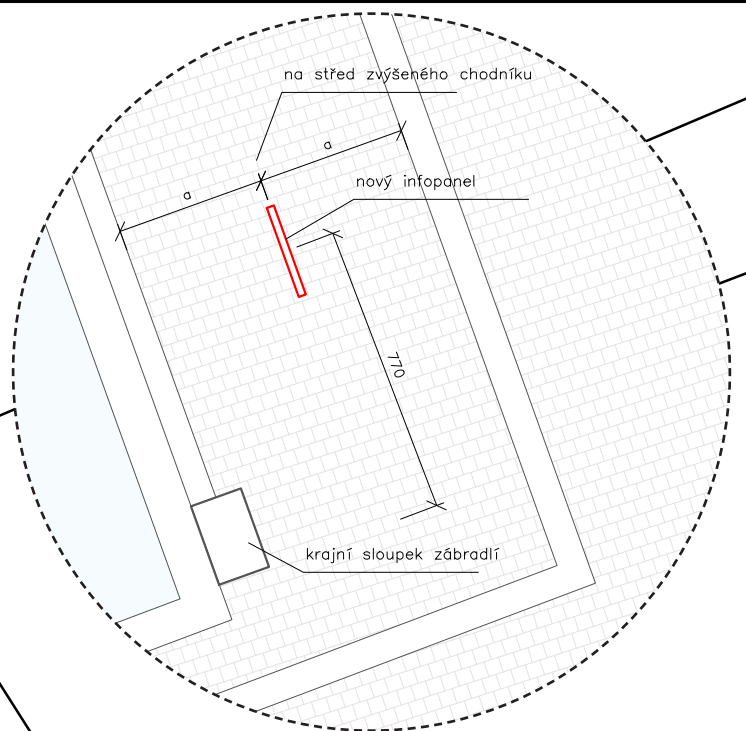
DETAIL M 1:20
