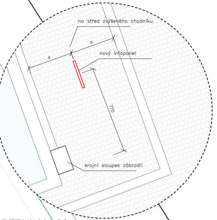
DETAIL M 1:20
